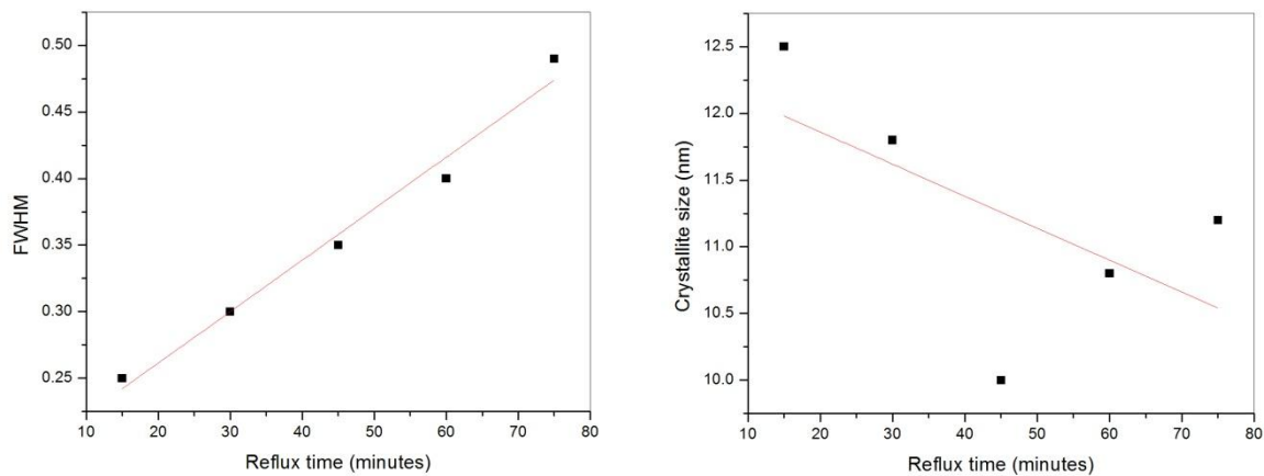
Fig. 2 (a) FWHM and (b) Crystallite size variation of CdS nanoparticles with different reflux time
