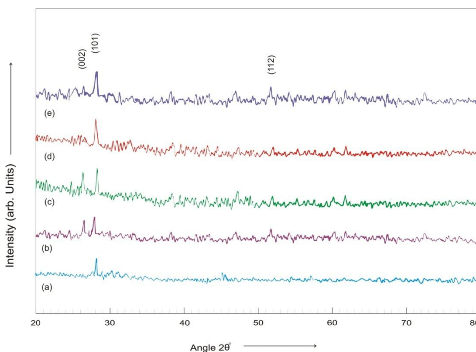
Fig. 1 XRD patterns of CdS nanoparticles at different reflux times
