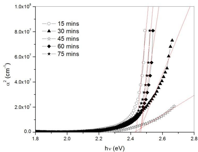
Fig. 5 Energy band gap plots of CdS nanoparticles for different reflux time
