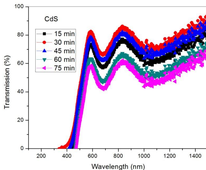
Fig. 4 Transmission spectra of CdS nanoparticles at different reflux times
