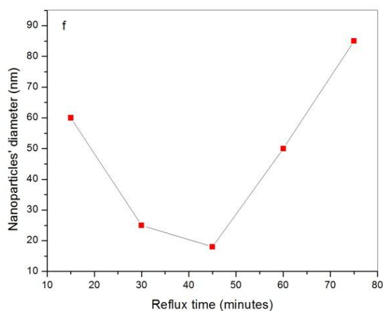
Fig. 3 SEM micrographs of CdS nanoparticles refluxed for (a) 15 min (b) 30 min (c) 45 min (d) 60 min (e) 75 min and (f) Plot between nanoparticles' size and Reflux time (min).
