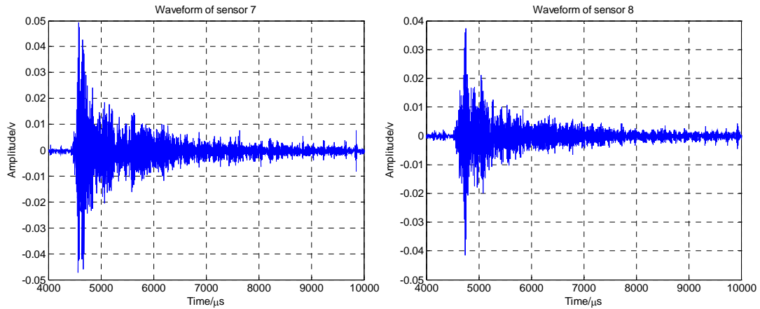
Fig.10 Waveform collected by sensor7 and sensor8
