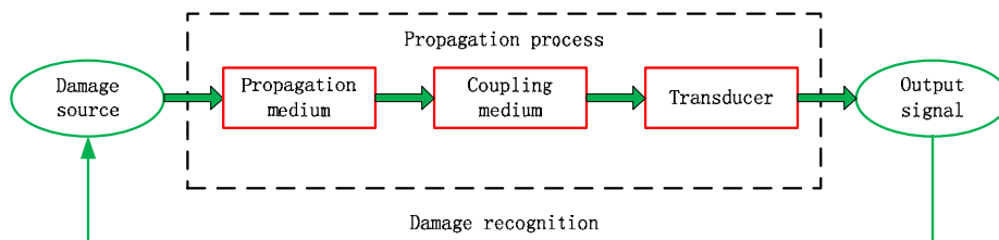
Fig.3 The whole process of AE monitoring
