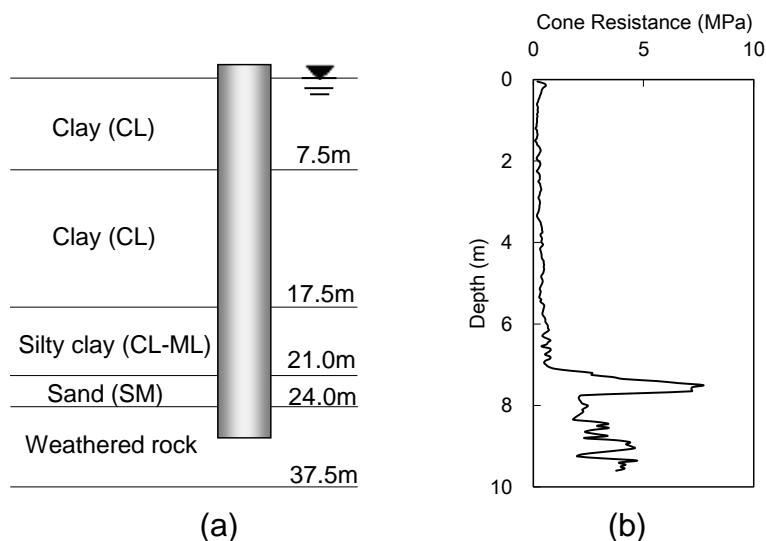
Fig. 4 Site condition and CPT results: (a) soil layer condition and (b) CPT profile.
