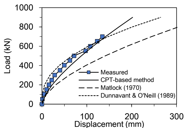
Fig. 5 Measured and calculated lateral load–pile head displacement curves.
