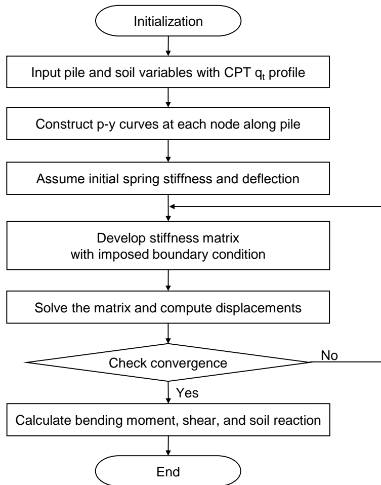
Fig. 3 Flow chart for CPT-based p-y analysis.
