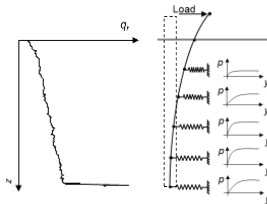
Fig. 1 Configuration of soil-spring model for laterally loaded pile.
