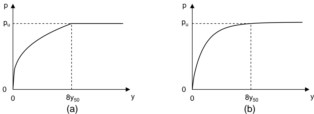
Fig. 2 p - y curves in clays by (a) Matlock (1970) and (b) Dunnivant and O'Neill (1989).
