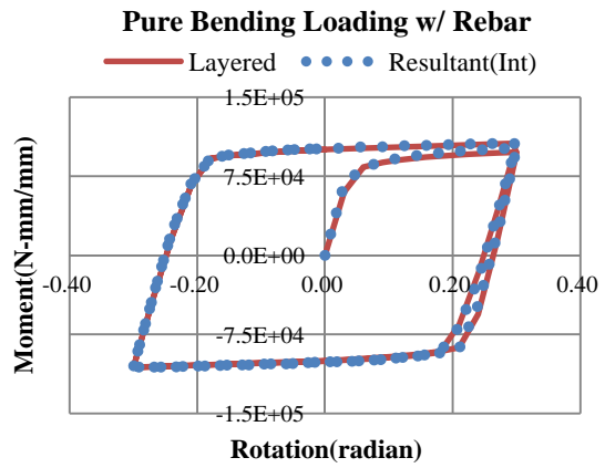
(b) Pure bending loading
