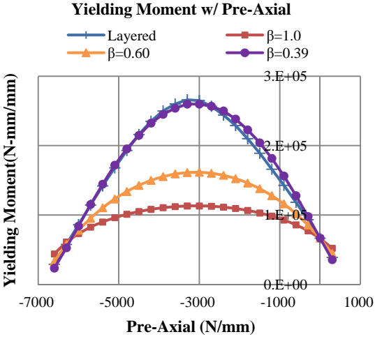
(b) Yielding moment with the exponent \beta
