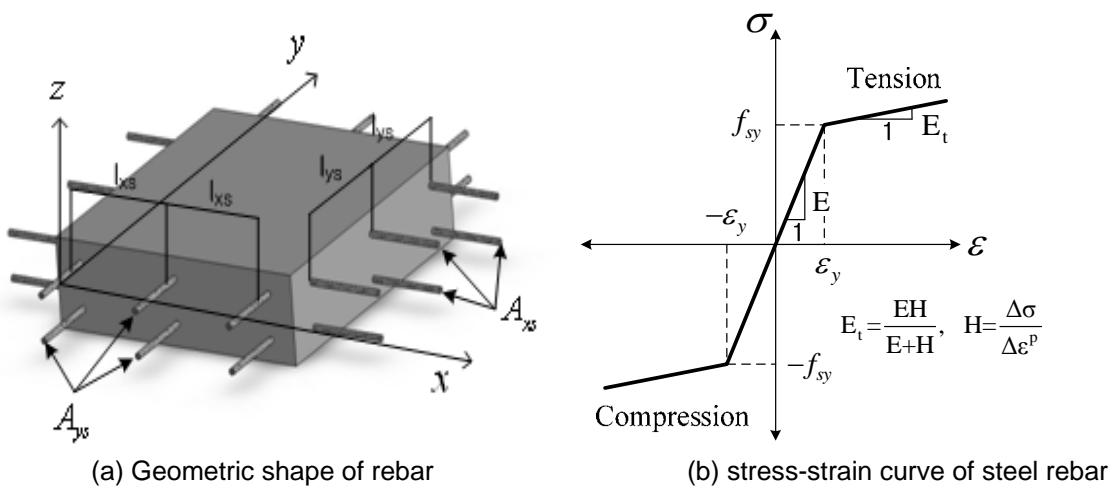
Figure 6 Geometric shape and stress-strain curve of a rebar
