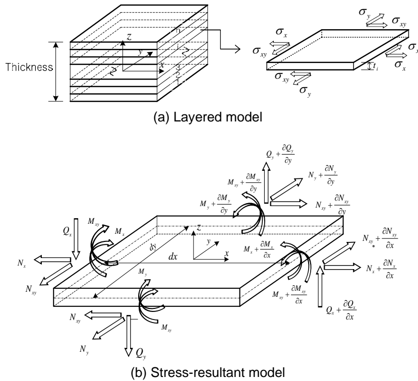
Figure 2 Local coordinate and nonlinear models for elasto-plastic behavior of plate
