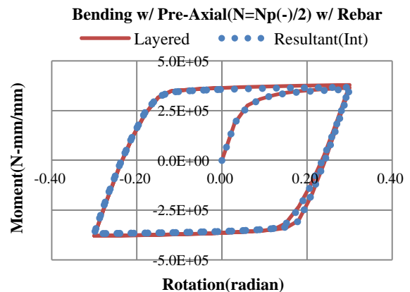
(b) Bending with pre-axial( 1/2N_p(-) ) w/ Rebar
