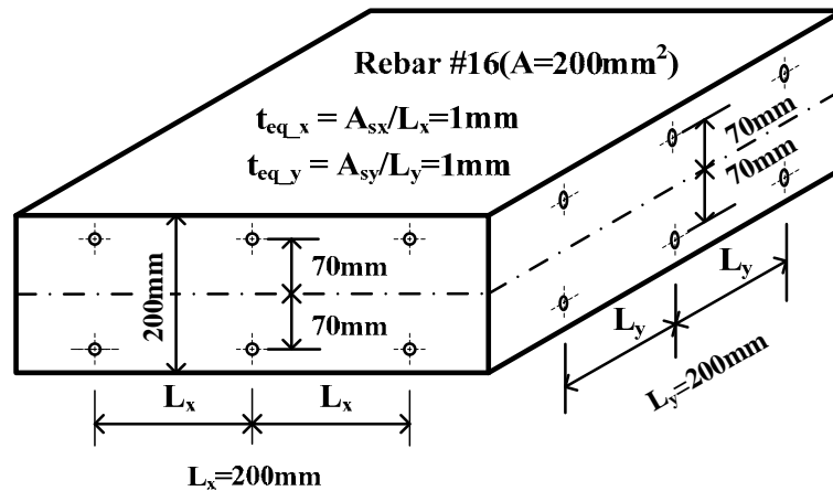
Figure 7 Geometry of a steel reinforced concrete plate
