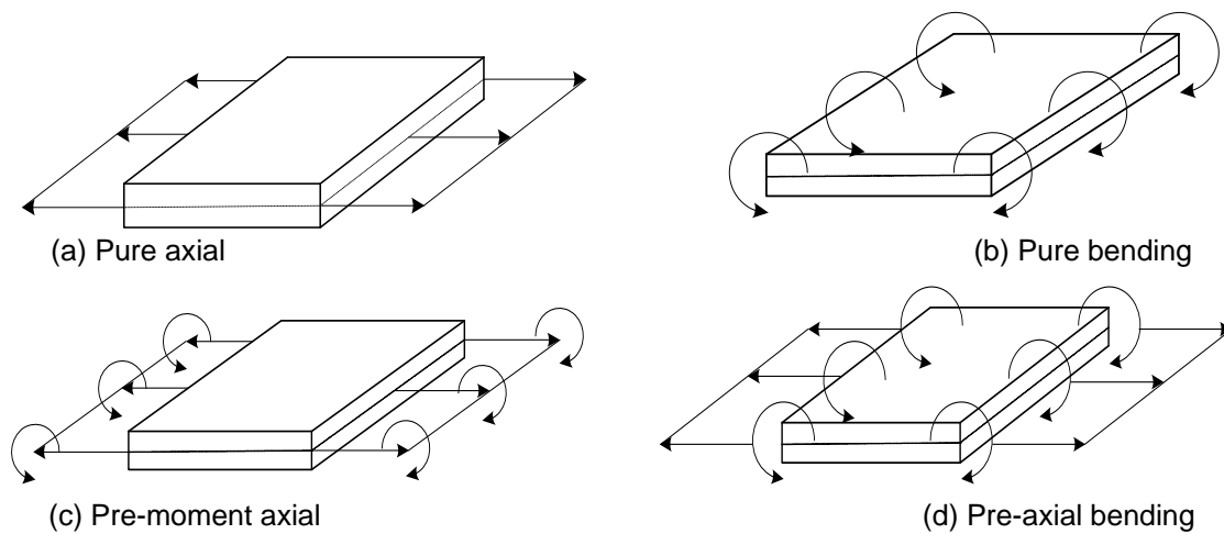
Figure 8 Test models of stress resultants yield criterion
