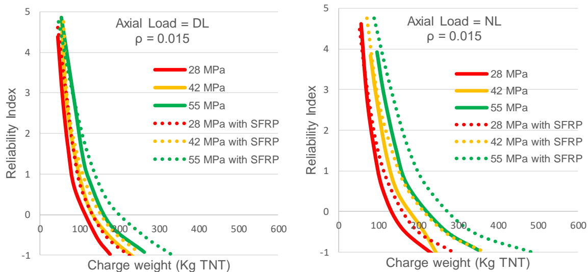
Fig. 1 Reliability results, 0.015 reinforcement ratio
