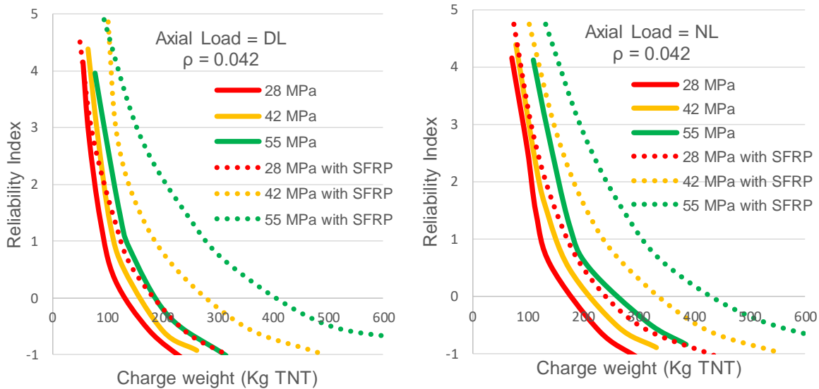
Fig. 2 Reliability Results, 0.042 reinforcement ratio
