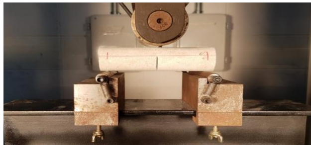
Fig. 1 The setup on the 3-point bending tests.
