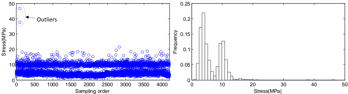
Fig. 7 Extracted peak stress sequences and stress histogram
