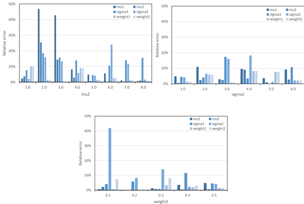
Fig. 4 Relative error: a) Cases 1-1 to 1-8; b) Cases 2-1 to 2-6; c) Cases 3-1 to 3-5
