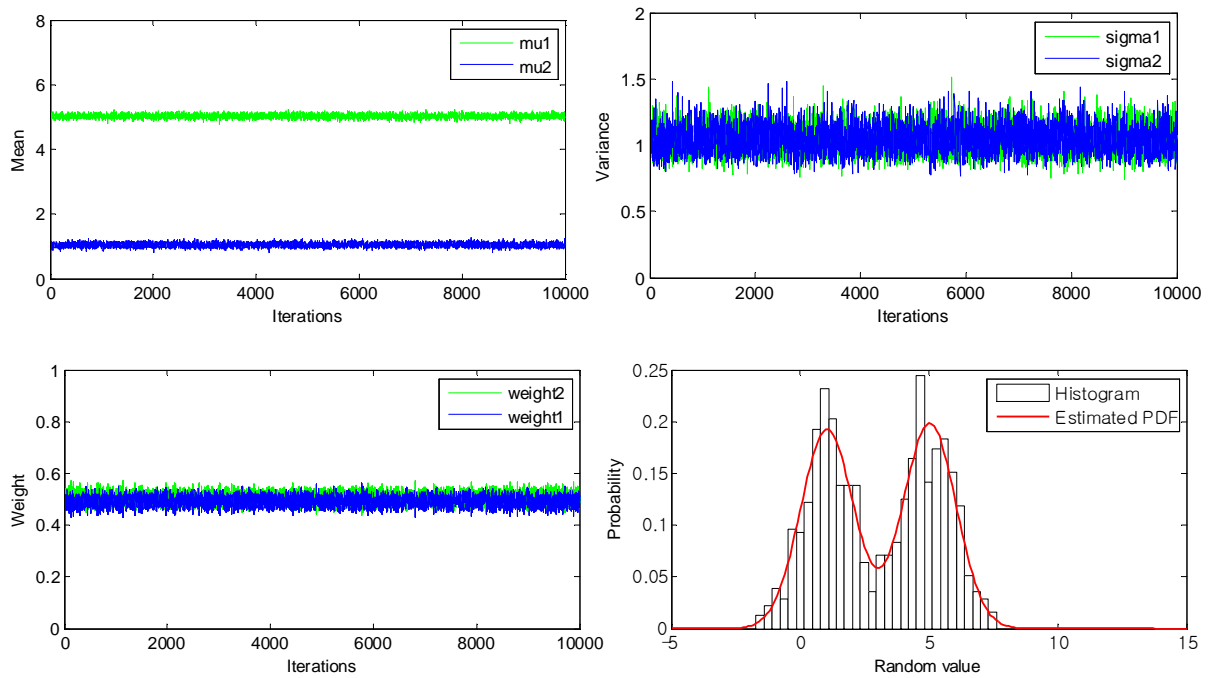
Fig. 3 Iteration paths for Case 1-5: a) iterations of component means; b) iterations of component variance; c) iterations of component weights; d) estimated PDF
