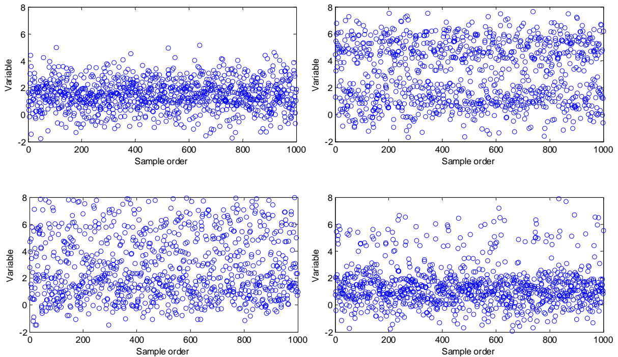
Fig. 2 Simulated random samples: a) Case 1-2; b) Case 1-5; c) Case 2-6; d) Case 3-1
