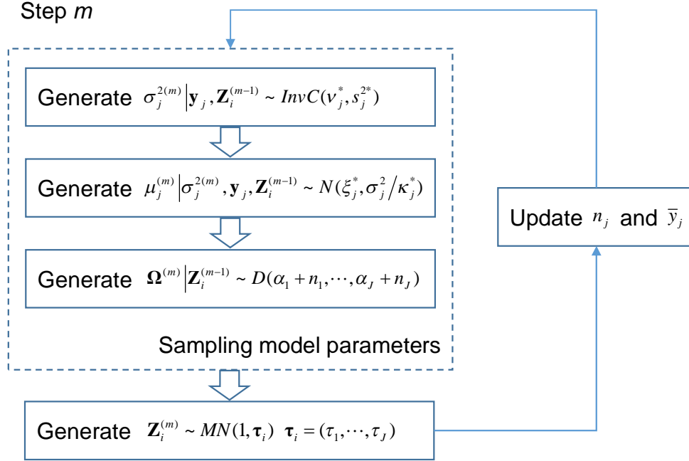
Fig. 1 Flowchart of Gibbs sampler for Gaussian mixture model
