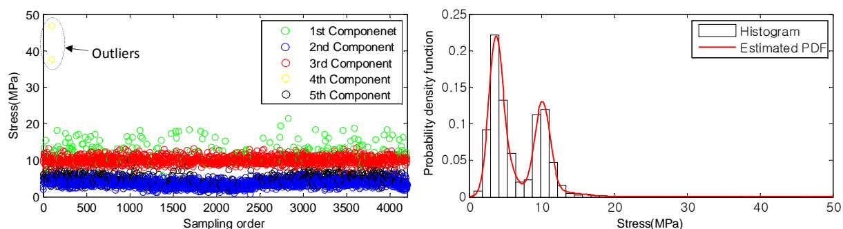
Fig. 9 Data cluster result and estimated PDF
