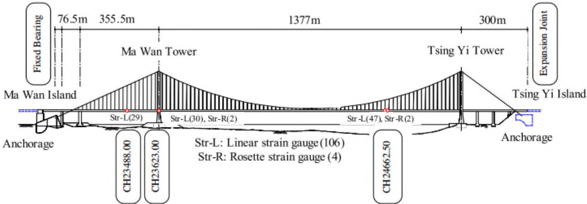
Fig. 5 TMB and strain monitoring sections
