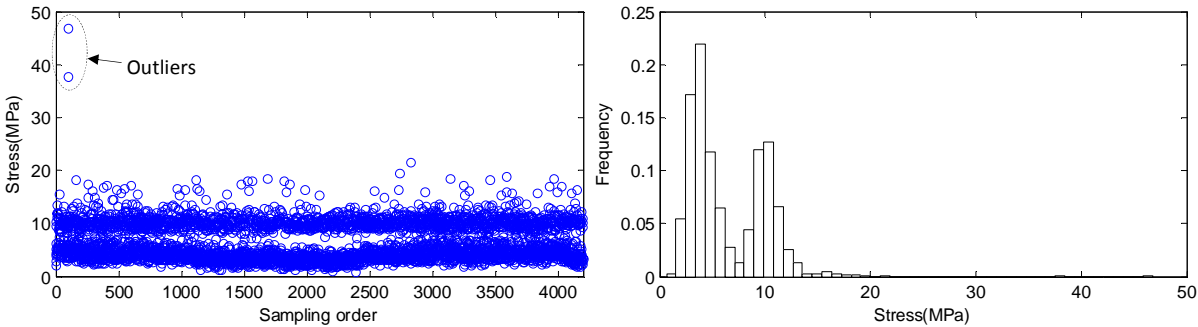
Fig. 7 Extracted peak stress sequences and stress histogram
