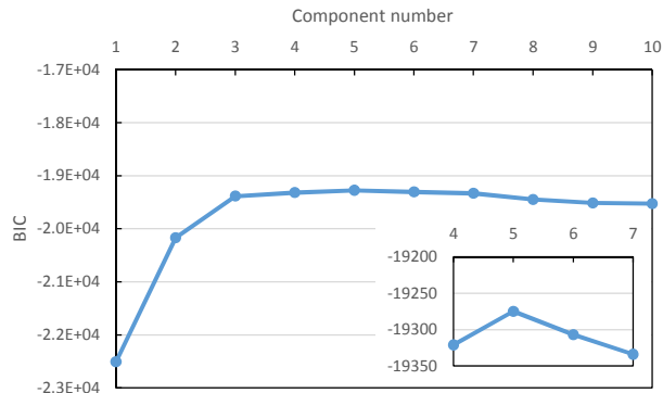
Fig. 8 Calculated BIC results
