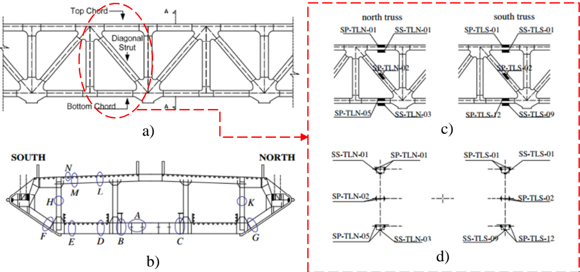
Fig. 6 Deck trusses of TMB and deployment of strain gauges
