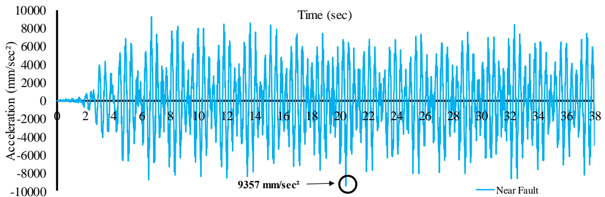
Fig. 11 Seismic accelerations on Point 11348 during near fault earthquake for structure with NSC (according to IBC 2003 standard).
