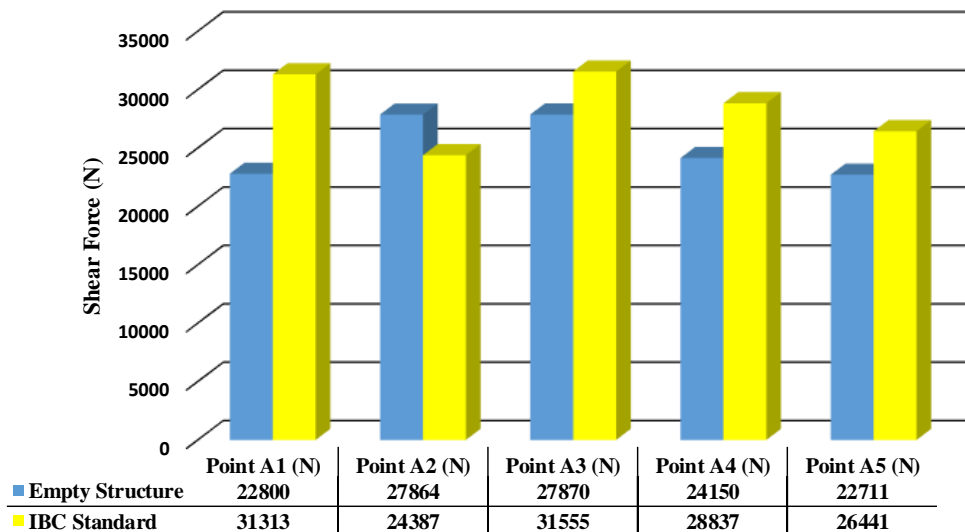
Fig. 8 Shear Forces along Axis A-A for near-fault earthquake.
