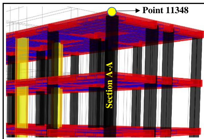
Fig. 9 View of the highest nodal point on section A-A.
