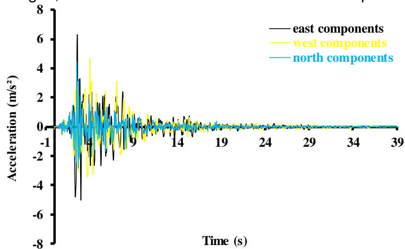
Fig. 5 Time History Graphics for Near Fault Ground Motions.
