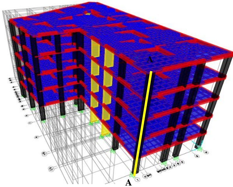
Fig. 3 3D model of RC structure.
