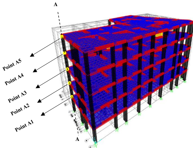
Fig. 6 View of A-A section of Structure.
