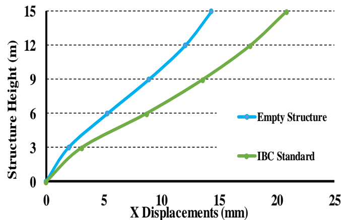
Fig. 7 Displacements along Axis A-A for Near-Fault earthquake.
