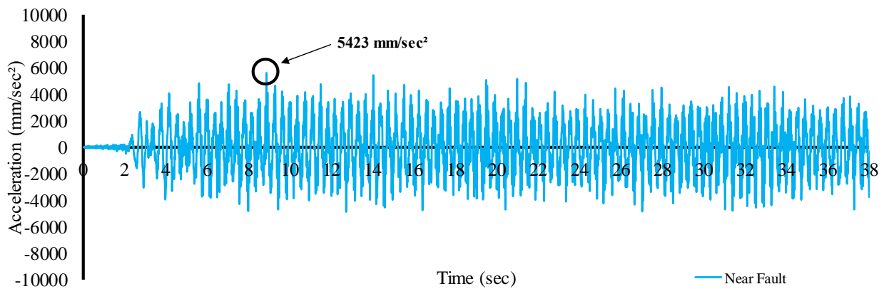
Fig. 10 Seismic accelerations on Point 11348 during near fault earthquake for structure without NSC.
